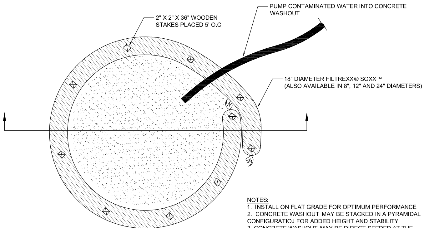
PLAN NTS
